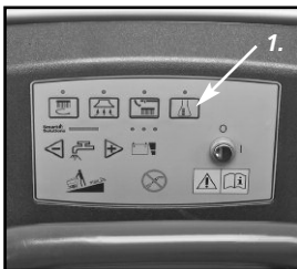
Easy to use control panel 1. Scrub 2. Vacuum 3. AXP on/off; set dilution rate at control panel
